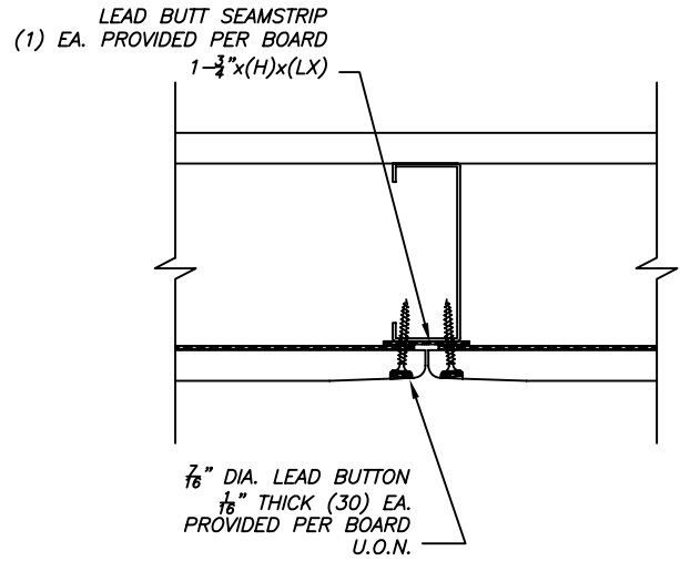
A-A - BUTT JOINT DETAIL
