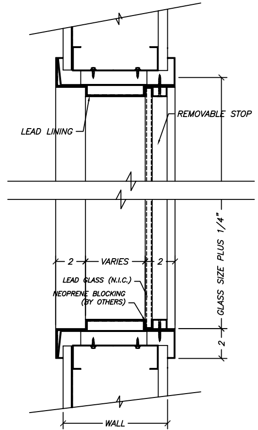
A-A LEADED JAMB DETAIL
